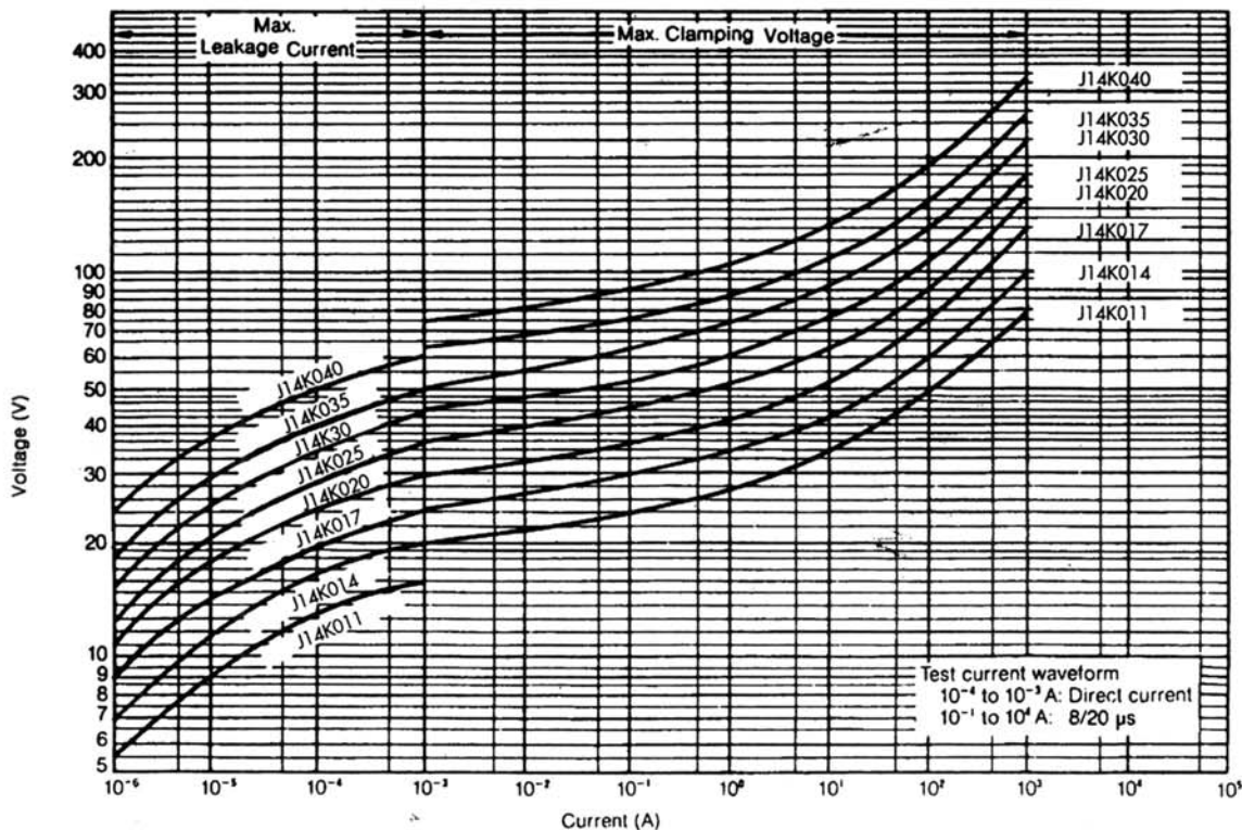
V-I Curve J14K011 to J14K040
