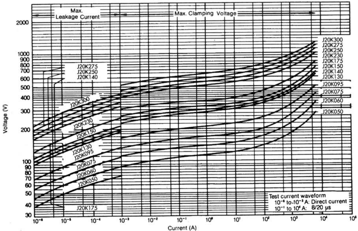
V-I Curve J20K050 to J20K300
