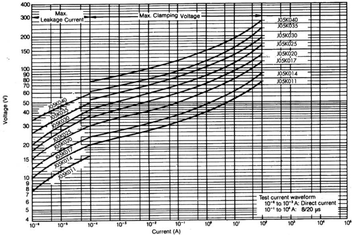
V-I Curve J05K050 to J05K300
