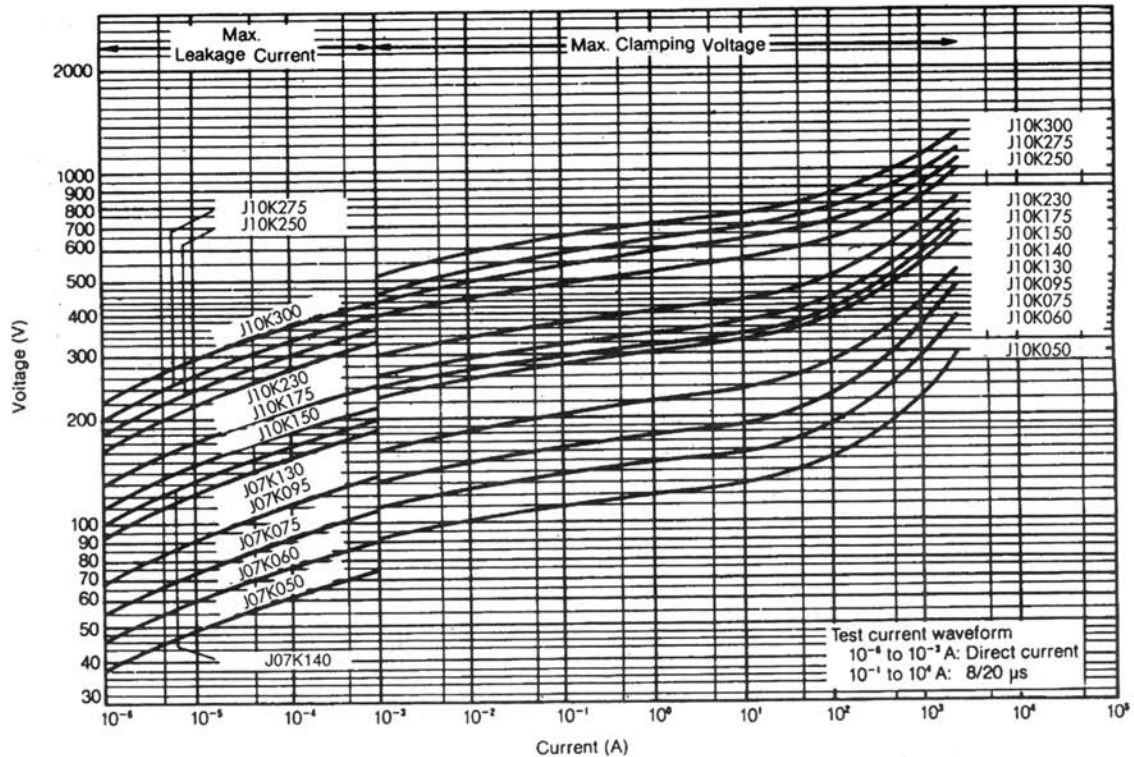
V-I Curve J10K050 to J10K300
