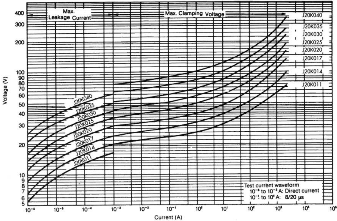
V-I Curve J20K011 to J20K040
