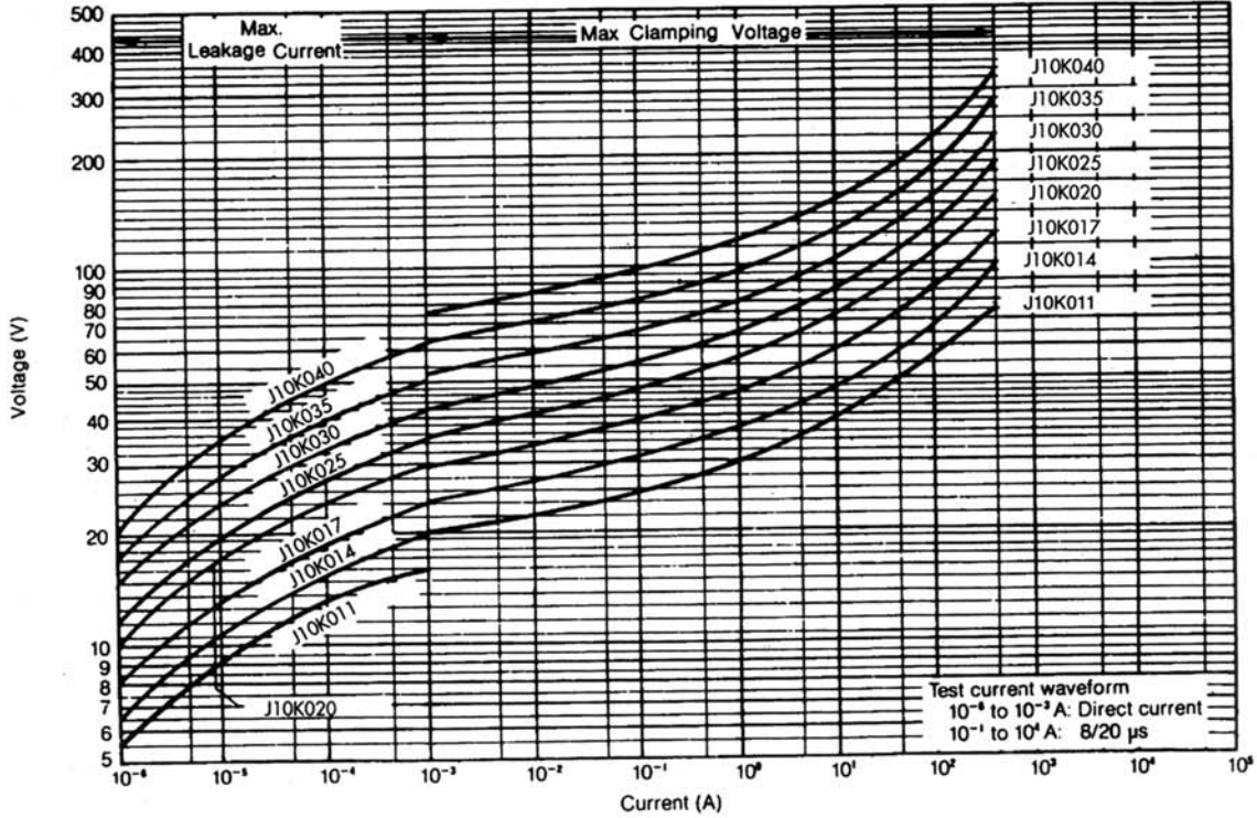
V-I Curve J10K011 to J10K040
